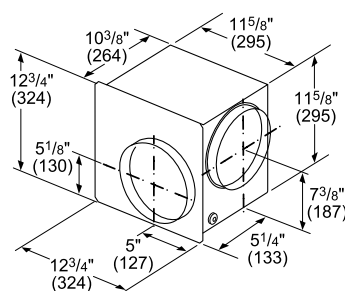
DHG602DUC 600 CFM Flexible Integral Blower – HDD Downdrafts
