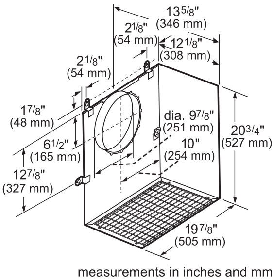
VTR2FZ-1000 CFM
