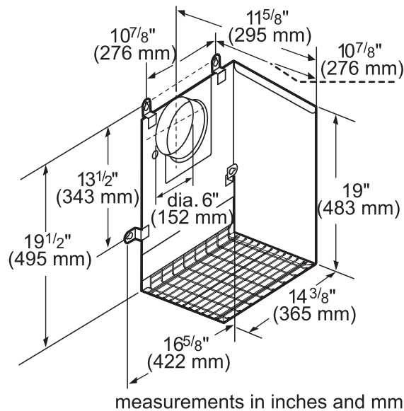
VTR1FZ-600 CFM
