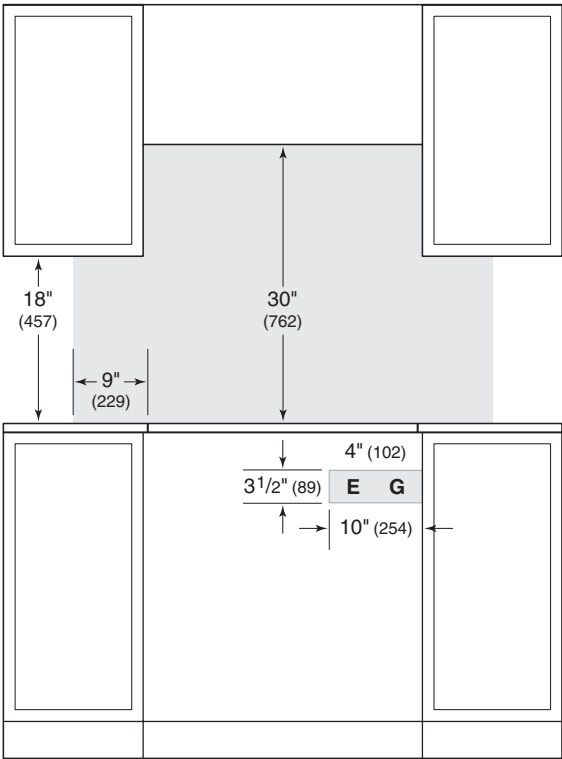
VISTA FRONTAL
